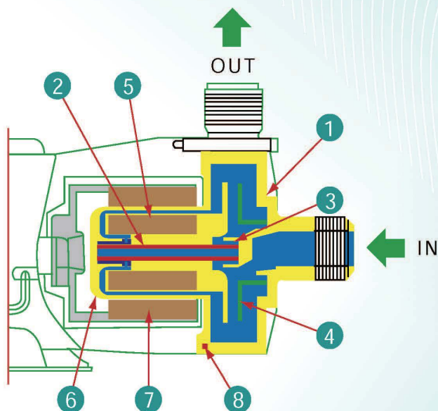
Structural Drawing :
