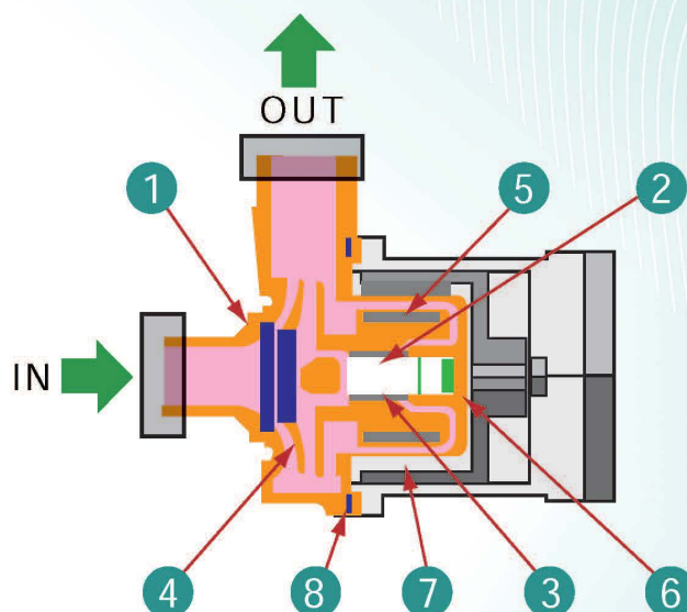
Structural Drawing :
